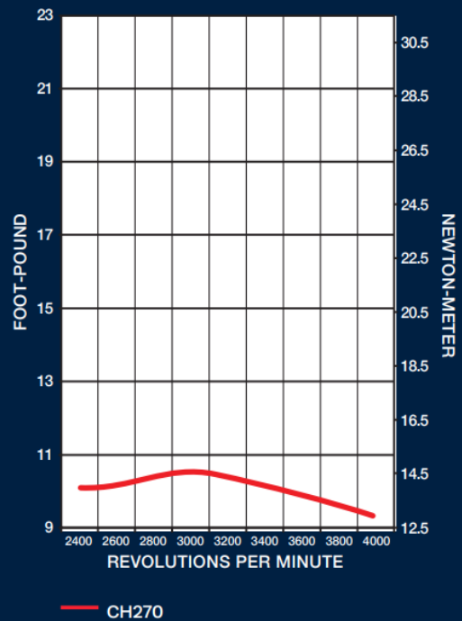
Maximum torque
