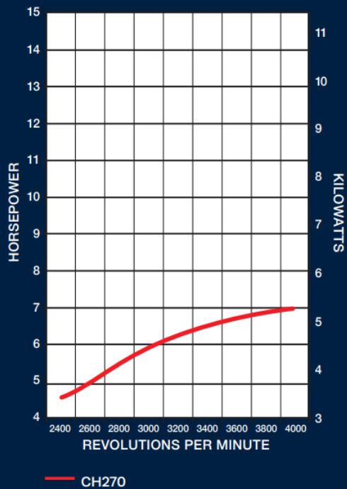
Maximum power
