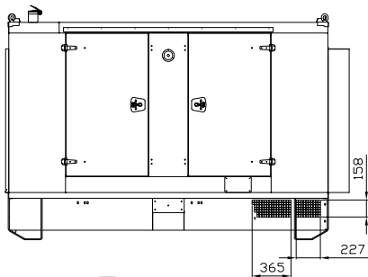
VISTA B VIEW
