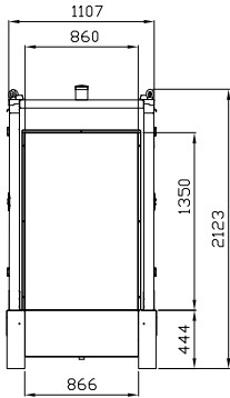
VISTA D VIEW
