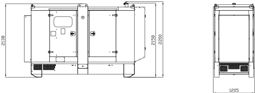
VISTA A VIEW
