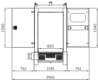
VISTA C VIEW
