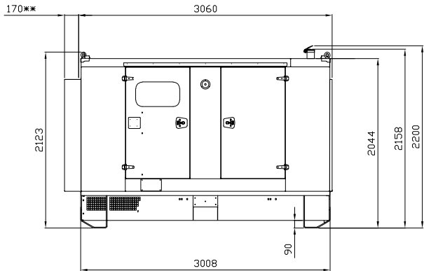
VISTA A VIEW
